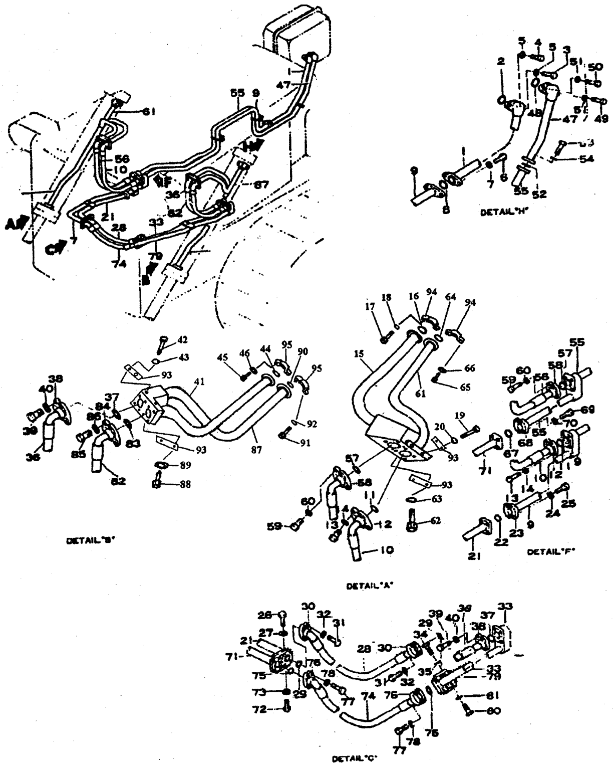
FIG 6126 HYDRAULIC PIPING (2/3)
