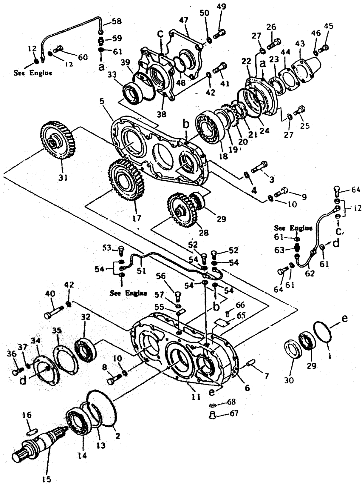
FIG. 1065 POWER TAKE OFF
