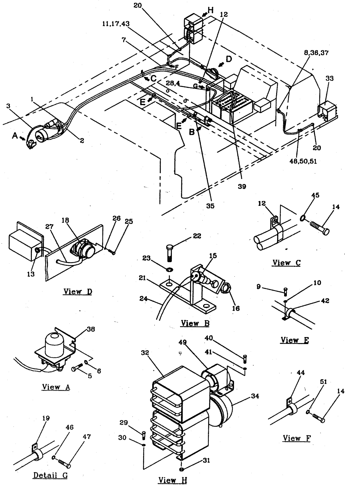
FIG. 1045B ELECTRICAL SYSTEM (2/2)
